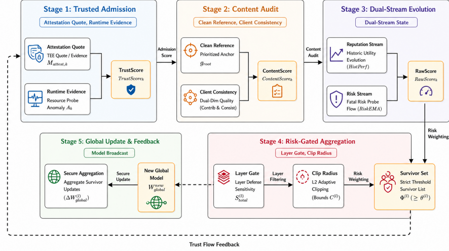
Fig. 3. Overview of the five-phase defense closed loop in trust-flow-driven trusted federated learning
