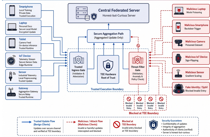
Fig. 2. Security penetration and multidimensional composite poisoning threat model in an edge wide-area network
